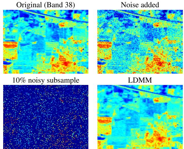
Fig. 2. Reconstruction of Indian Pine from 10% noisy subsample.
