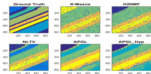
Fig. 5. Algorithms run on Salinas-A Dataset with 10% Pixels Replaced by Noise
