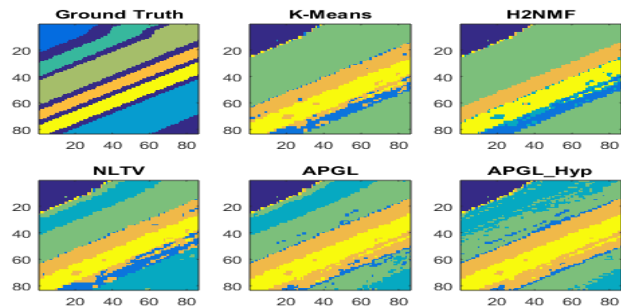
Fig. 4. Algorithms run on Original Salinas-A Dataset
