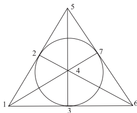
FIGURE 6. Fano plane
