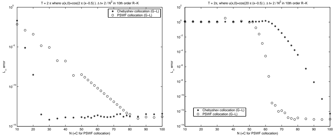
Figure 9: L_\infty -error from solving u_t = u_x with a collocation method and strongly imposed boundary condition. Final time: T = 2\pi . 10th order RK with \Delta t = \frac{2}{N^2} . Left: u(x, t) = \cos(2\pi(x - 0.5 + t)) ; Right: u(x, t) = \cos(20\pi(x - 0.5 + t)) . 'o': PSWF; '*' : Chebyshev.
