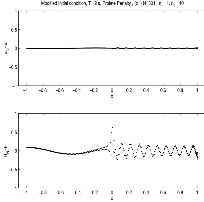
Figure 16: Pointwise errors with the initial conditions computed from the numerical scheme.
