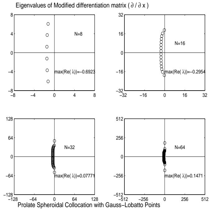
Figure 11: Eigenvalues of the differentiation matrix for the PSWF collocation method. Boundary condition is imposed strongly.
