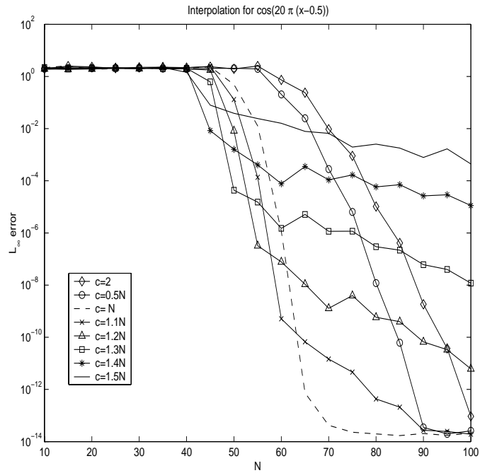
Figure 5: The loss of accuracy as c approaches \frac{\pi}{2}N .
