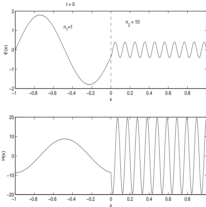
Figure 13: Exact solution at t = 0 , n_1 = 1.0 , n_2 = 10.0 . Upper: electric field E(x, t) ; Lower: magnetic field H(x, t)
