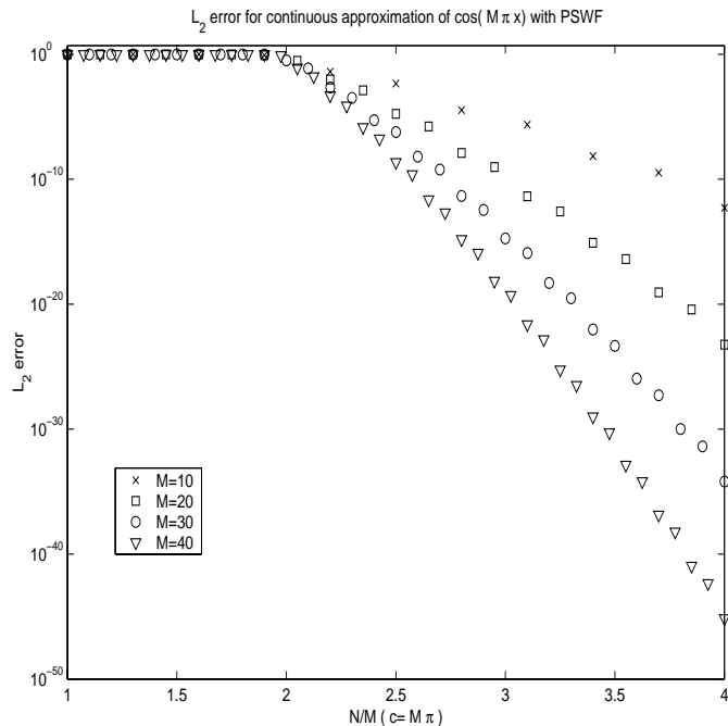
Figure 2: L^2 -error of the PSWF expansion (truncated after N terms) of \cos(M\pi x) versus N/M . \times : M = 10 ; \square : M = 20 ; \circ : M = 30 ; \nabla : M = 40 .
