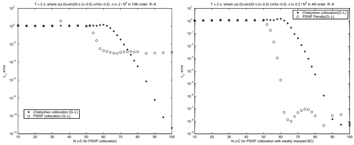
Figure 10: L_\infty -error of solving u_t = u_x by collocation methods. u(x, 0) = \sin(20\pi(x - 0.5)) + H(x - 0.5) . Final time: T = 2\pi . Left: Chebyshev and PSWF collocation method with Strongly imposed boundary condition. Right: PSWF collocation method with weakly imposed boundary condition.
