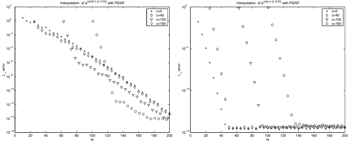
Figure 3: Demonstration that the optimal c , if it exists, depends on the specific problem and the required accuracy. Left: L_\infty error for the interpolation of e^{\cos(5\pi(x-0.5))} . For an error around 10^{-6} , c = 100 is the best choice. For an error as small as 10^{-10} , c = 160 is optimal. Right: L_\infty -error for the interpolation of e^{\cos(\pi(x-0.5))} . Clearly, c = 0 (Legendre basis) is the best among the four choices.
