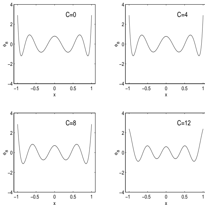
Figure 1: \psi_8^c(x) for different values of c
