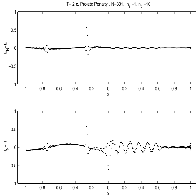
Figure 15: Pointwise error from the PSWF collocation method. c = N = 301 . t = 2\pi . Upper: electric field; Lower: magnetic field.
