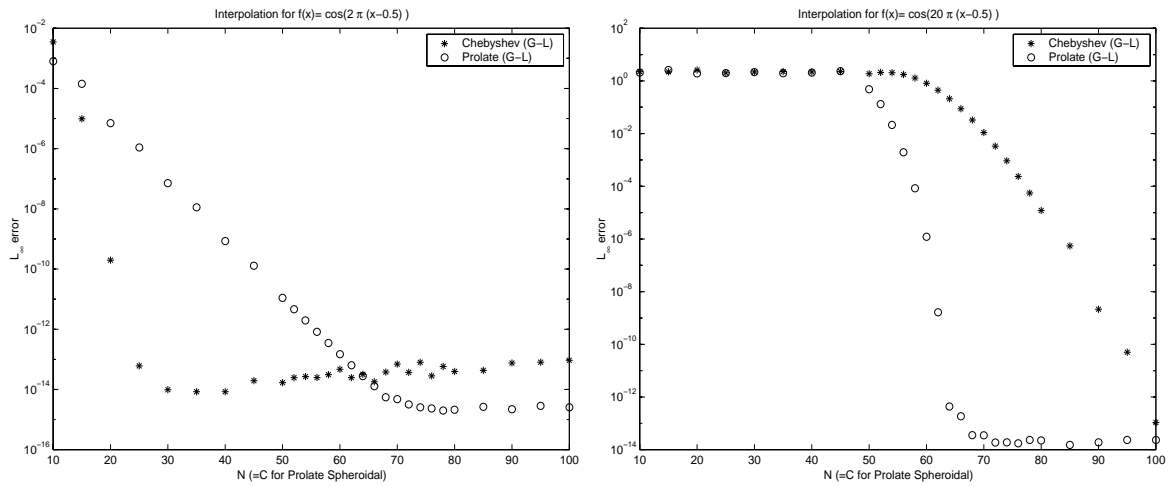
Figure 6: Interpolation results. 'o': Prolate spheroidal wave basis; '*' : Chebyshev polynomials basis. c = N for prolate spheroidal wave basis. Left: f(x) = \cos(2\pi(x - 0.5)) ; Right: f(x) = \cos(20\pi(x - 0.5))
