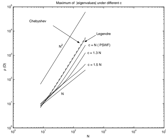
Figure 7: The largest absolute eigenvalue of the PSWF collocation method using different values of c , and the Chebyshev and Legendre collocation method.
