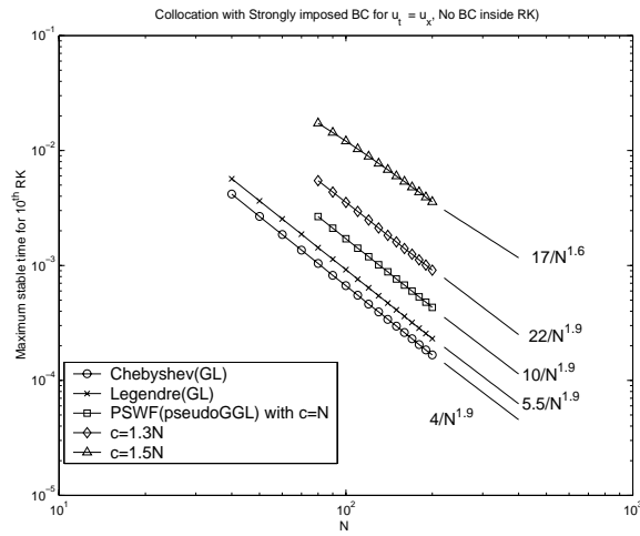
Figure 8: The largest stable time-step for the PSWF collocation method using different values of c 's, the Chebyshev and Legendre collocation method. A 10th order explicit Runge-Kutta scheme was used.
