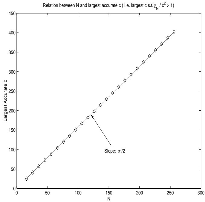
Figure 4: Computational validation of the relation between N and the biggest c which makes q_N \leq 1 . The slope is \pi/2 as predicted in the text.
