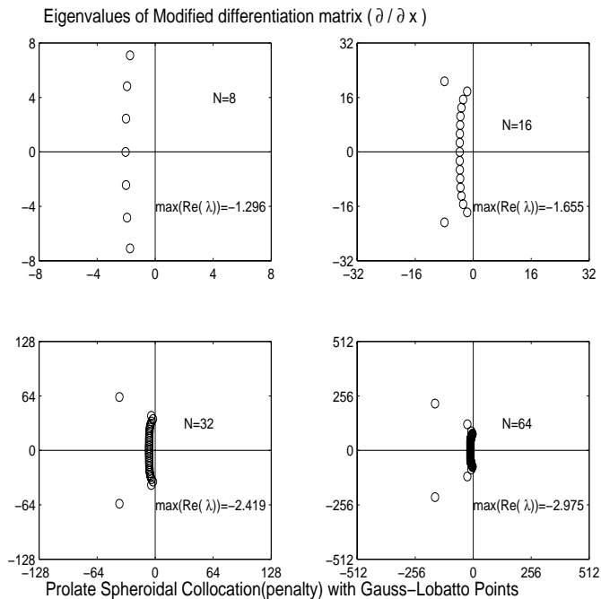
Figure 12: Eigenvalues of the differentiation matrix for the PSWF collocation method. Boundary condition is imposed weakly.
