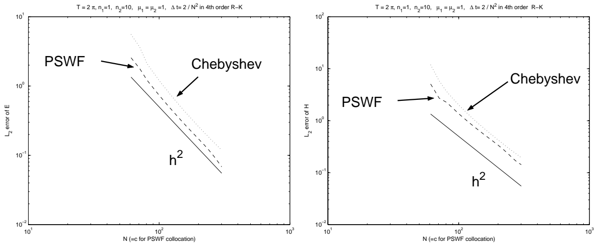
Figure 14: The discrete L_2 -error at t = 2\pi . Strongly imposed boundary condition for the Chebyshev collocation method, weakly imposed boundary condition for the PSWF collocation method. Left: electric field E(x, t) ; Right: magnetic field H(x, t) .
