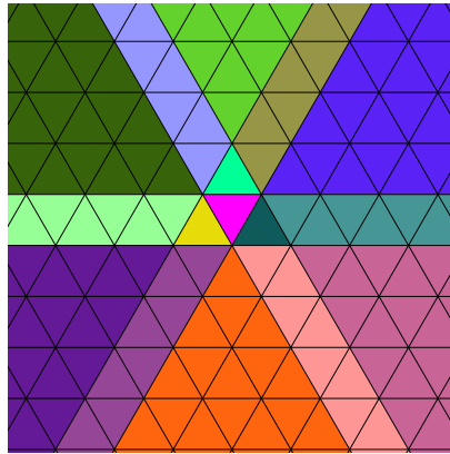
FIGURE 1. The regions in \mathcal{R}_0 for \tilde{A}_2
