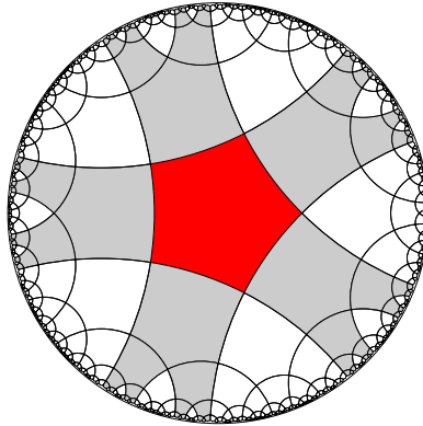
FIGURE 7. Cells for a hyperbolic Coxeter group
