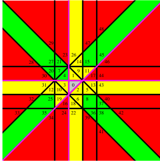
FIGURE 4. States for the automaton accepting \text{Red}(\tilde{C}_2) built using \mathcal{R}_v
