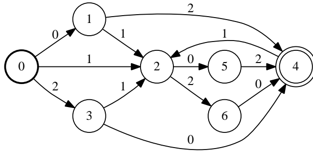
FIGURE 6. The minimal automaton accepting \text{Red}(C)
