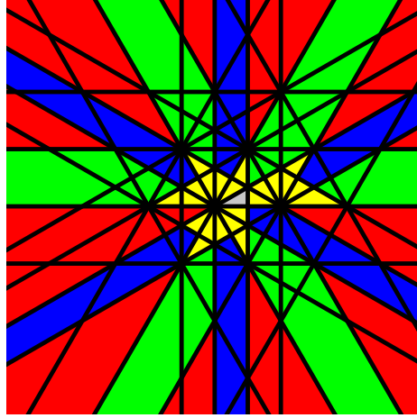
FIGURE 2. The left cells of \tilde{G}_2 and the regions in \mathcal{R}_1
