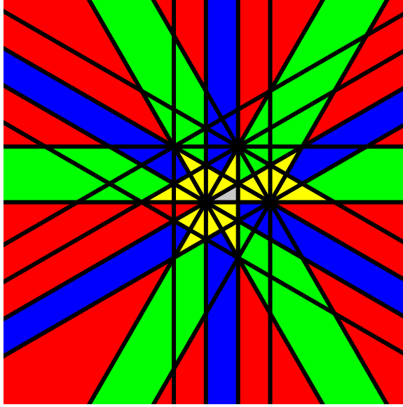
FIGURE 3. The regions in \mathcal{R}_\nu for \tilde{G}_2
