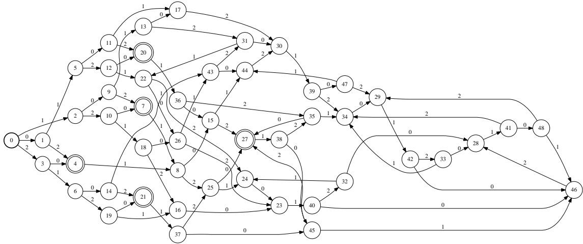
FIGURE 5. The automaton built from Figure 4
